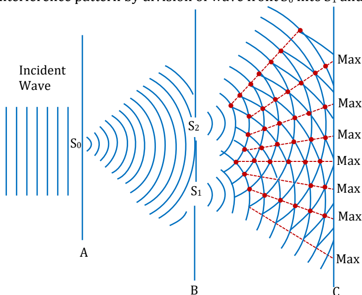
Figure: Young's arrangement to produce stationary interference pattern by division of wave front S_0 into S_1 and S_2
