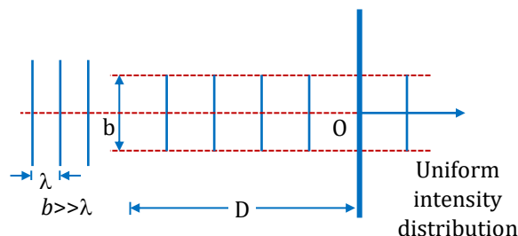
(A) Size of the slit is very large compared to wavelength
