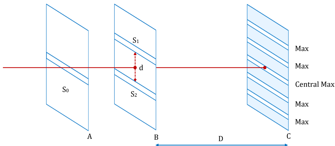
Figure: Young's arrangement to produce stationary interference pattern by division of wave front S_0 into S_1 and S_2
